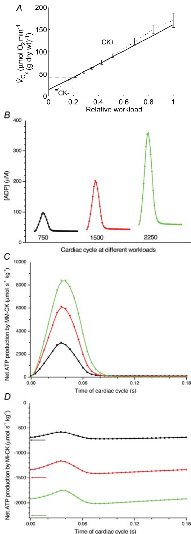
Figure 4. Mathematical modelling of the regulation of mitochondrial respiration in cardiac cells in vivo under physiological conditions controlled by the Frank-Starling mechanism
